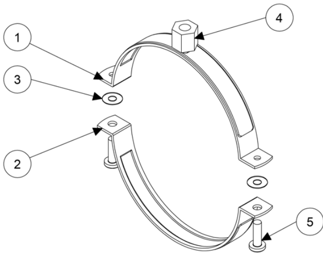
EXPLODED VIEW
