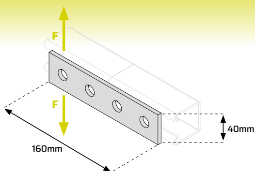
Splice Plate 4-Hole
