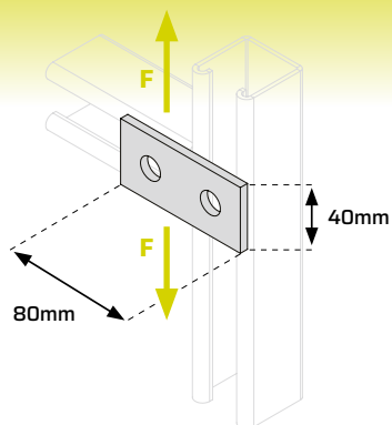
Splice Plate 2-Hole
